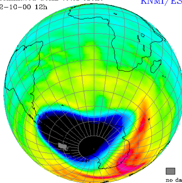
Assimilated GOME total ozone 12-10-00 12h
